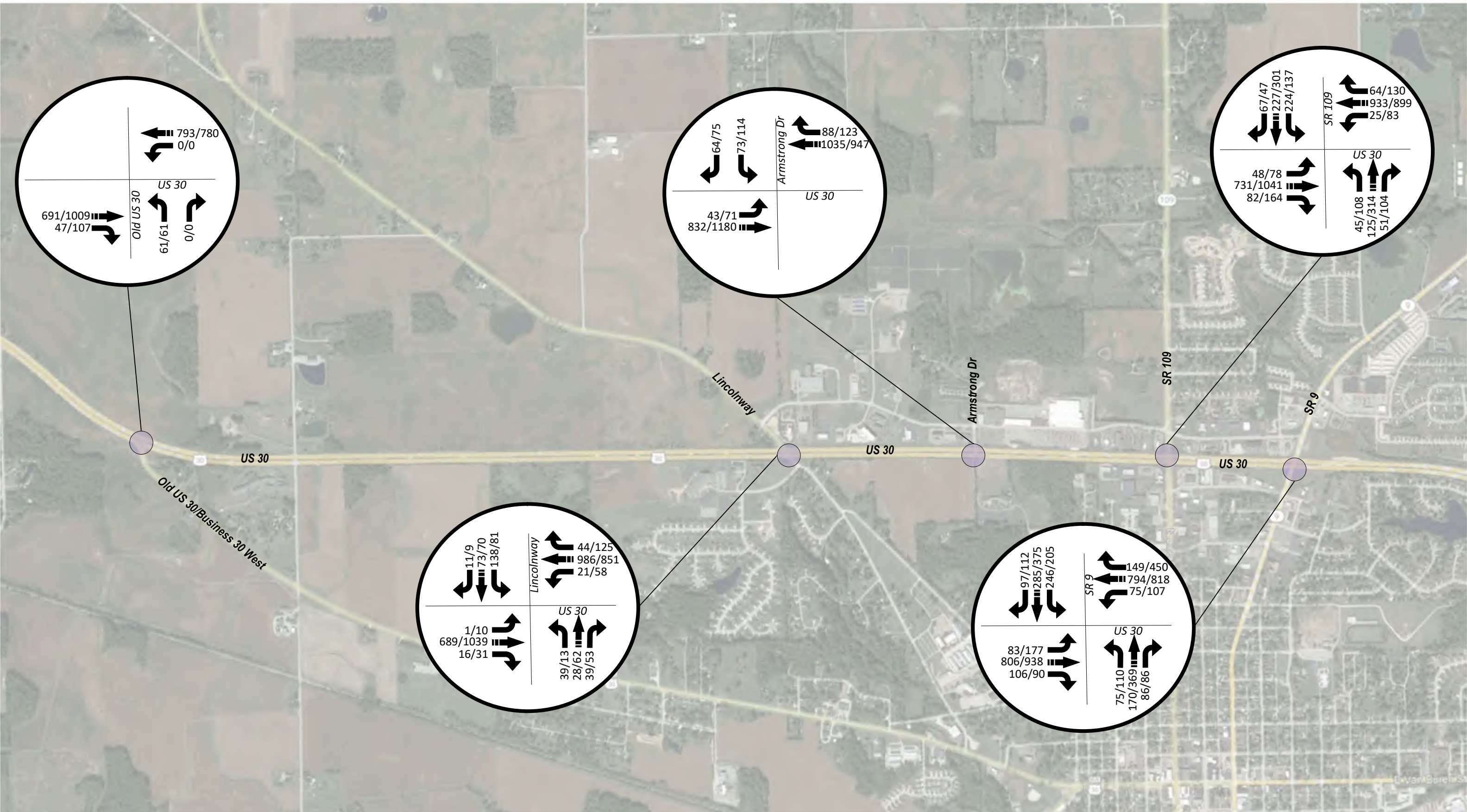
ProPEL US 30 East Whitley County – 2 of 4 Proposed (2045) Traffic Volumes ##/## = AM Peak Hour / PM Peak Hour
