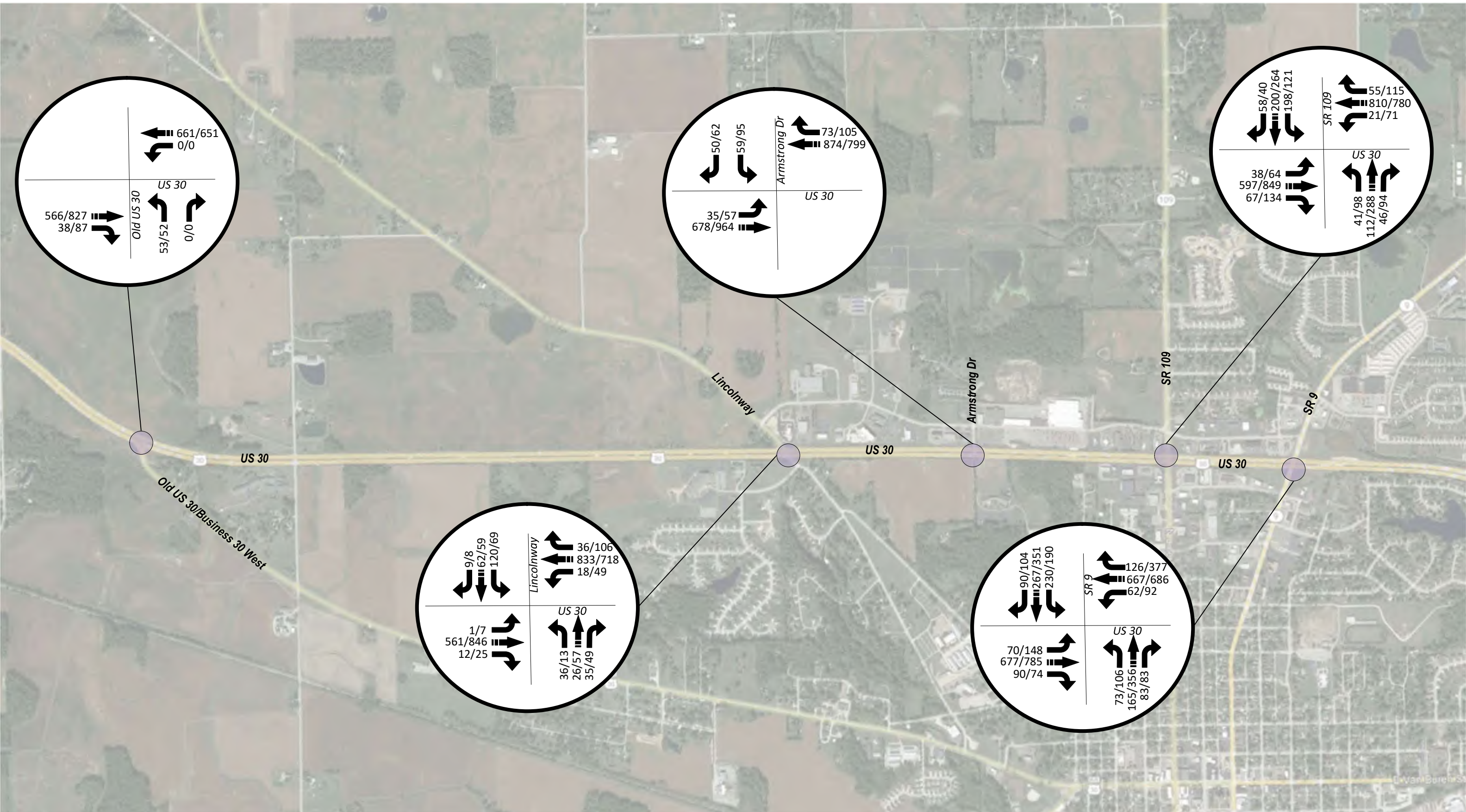
ProPEL US 30 East Whitley County – 2 of 4 Existing (2022) Traffic Volumes ##/## = AM Peak Hour / PM Peak Hour
