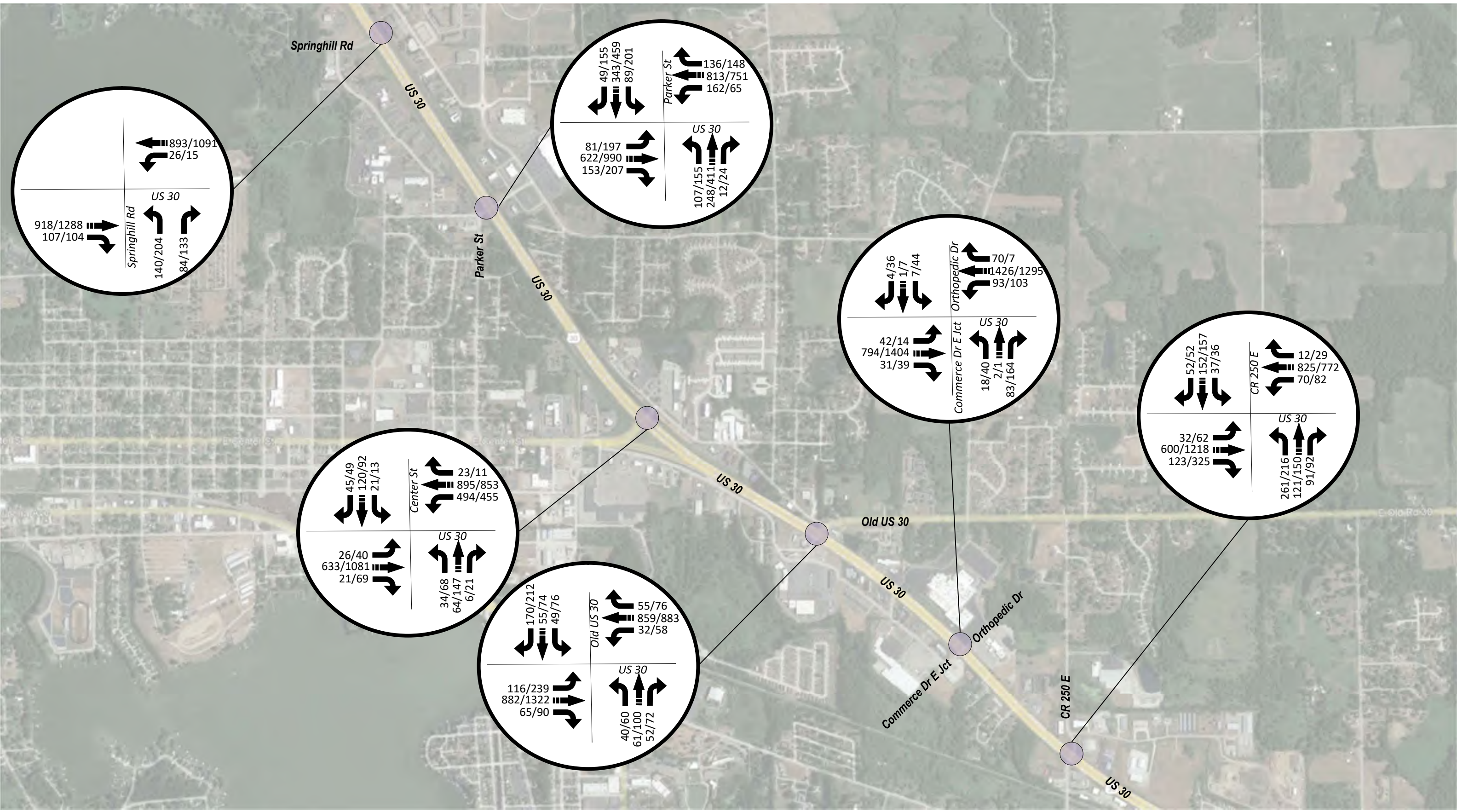
ProPEL US 30 East Kosciusko County – 3 of 4 Proposed (2045) Traffic Volumes ##/## = AM Peak Hour / PM Peak Hour
