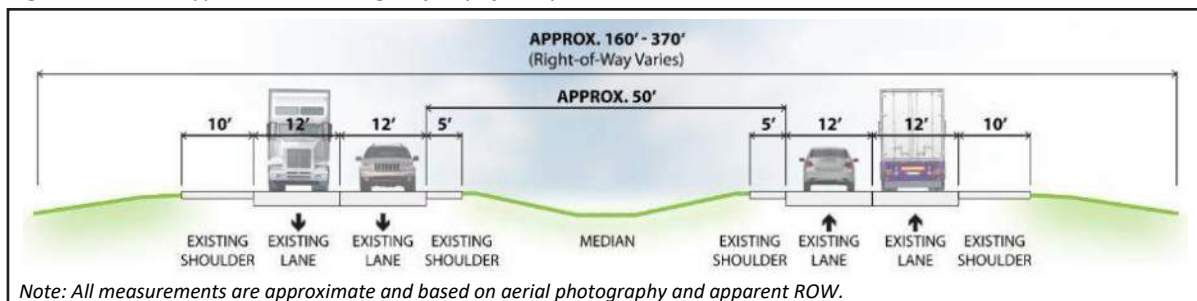
Figure 3-1: US 31 Typical Section Along Majority of Study Corridor
