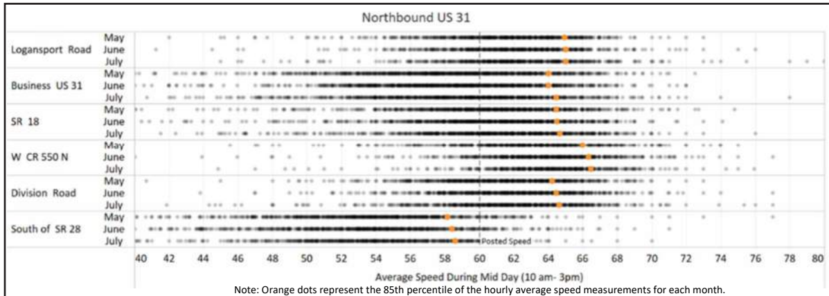
Figure 6-15: Northbound US 31 - Average Hourly Speeds Between 10 AM and 3 PM (Heavy Vehicles)
