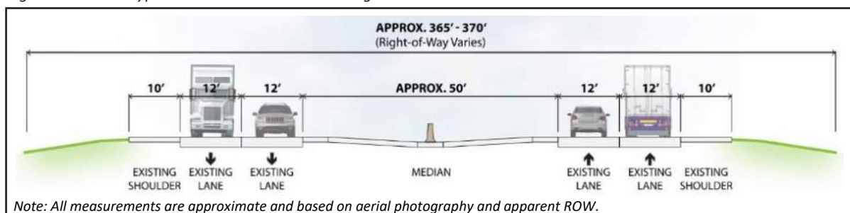
Figure 3-2: US 31 Typical Section at US 24 Interchange
