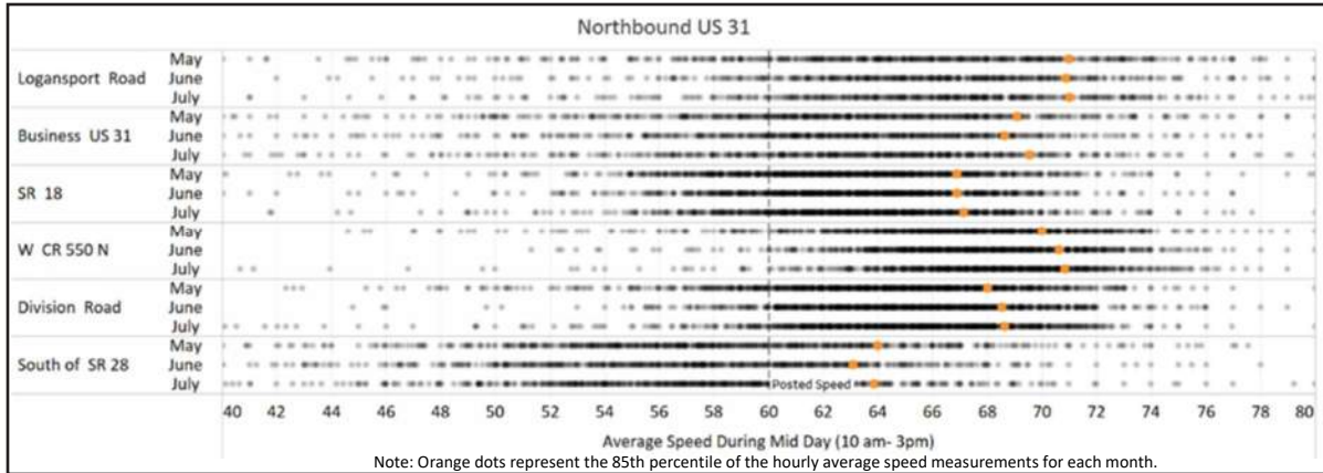
Figure 6-13: Northbound US 31 - Average Hourly Speeds Between 10 AM and 3 PM (Passenger Vehicles)
